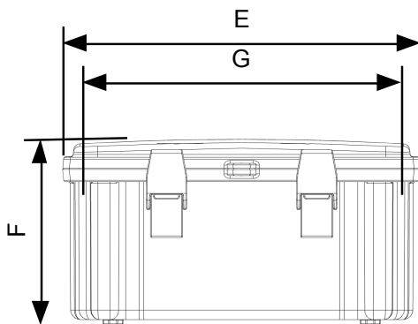
Dimensions (inches)
